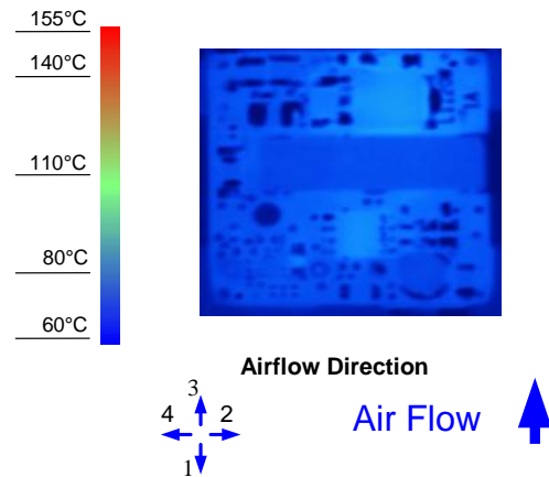
Figure 8. Thermal Image for Airflow Direction 3 (1A output, 55°C ambient, 200 LFM, typical Vin, open frame, unit soldered onto a fixture board)
